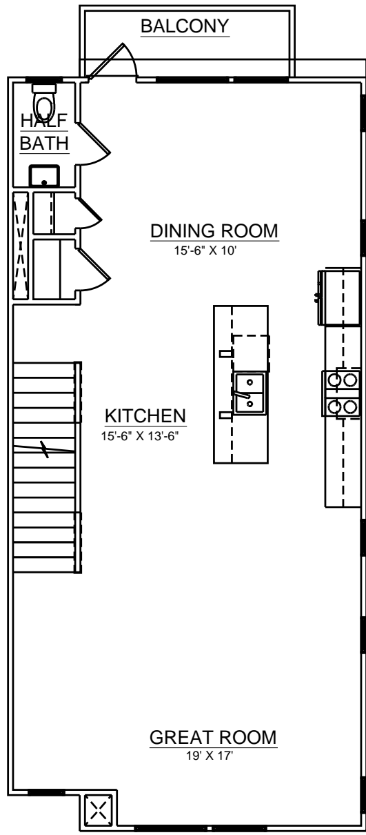
SECOND FLOOR
