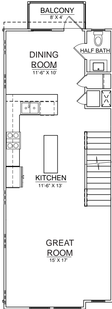
MAIN FLOOR
