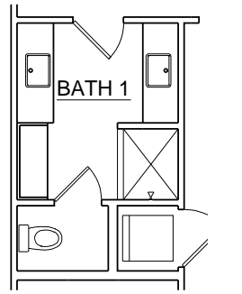
OPT. BATHROOM 1 LAYOUT
