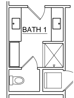
OPT. BATHROOM 1 LAYOUT
