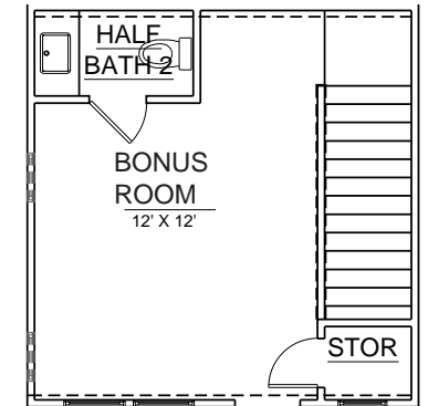
OPT. HALF BATHROOM IN BONUS ROOM
