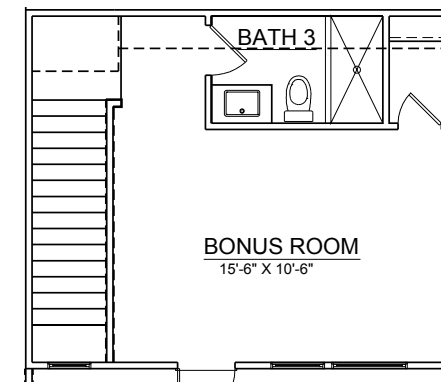
OPT. FULL BATHROOM IN BONUS ROOM
