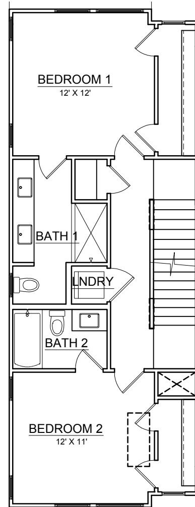
SECOND FLOOR
