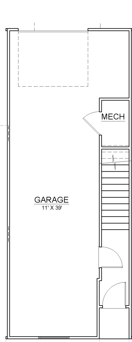
GROUND FLOOR
