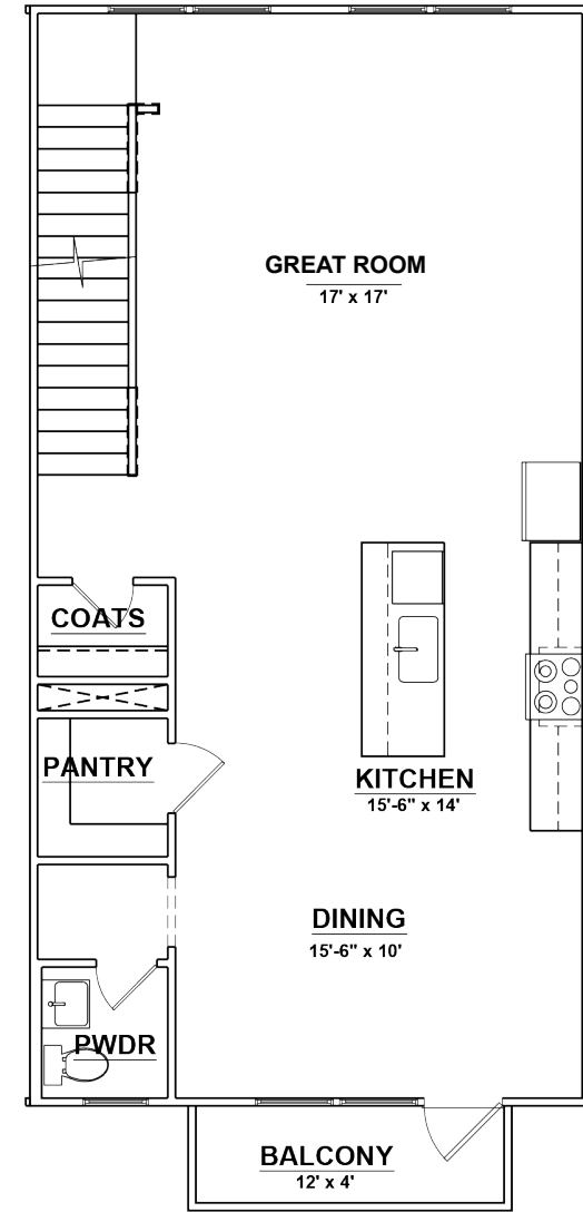
MAIN FLOOR
