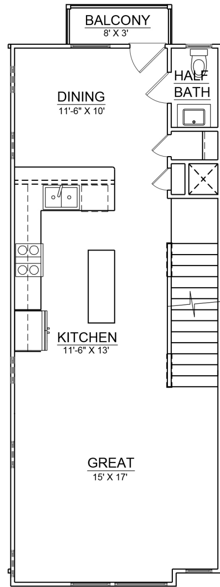
MAIN FLOOR
