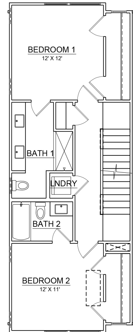
THIRD FLOOR WITH ROOFTOP OPTION
